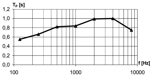
Fig. 2 RT of the measured auditory room
